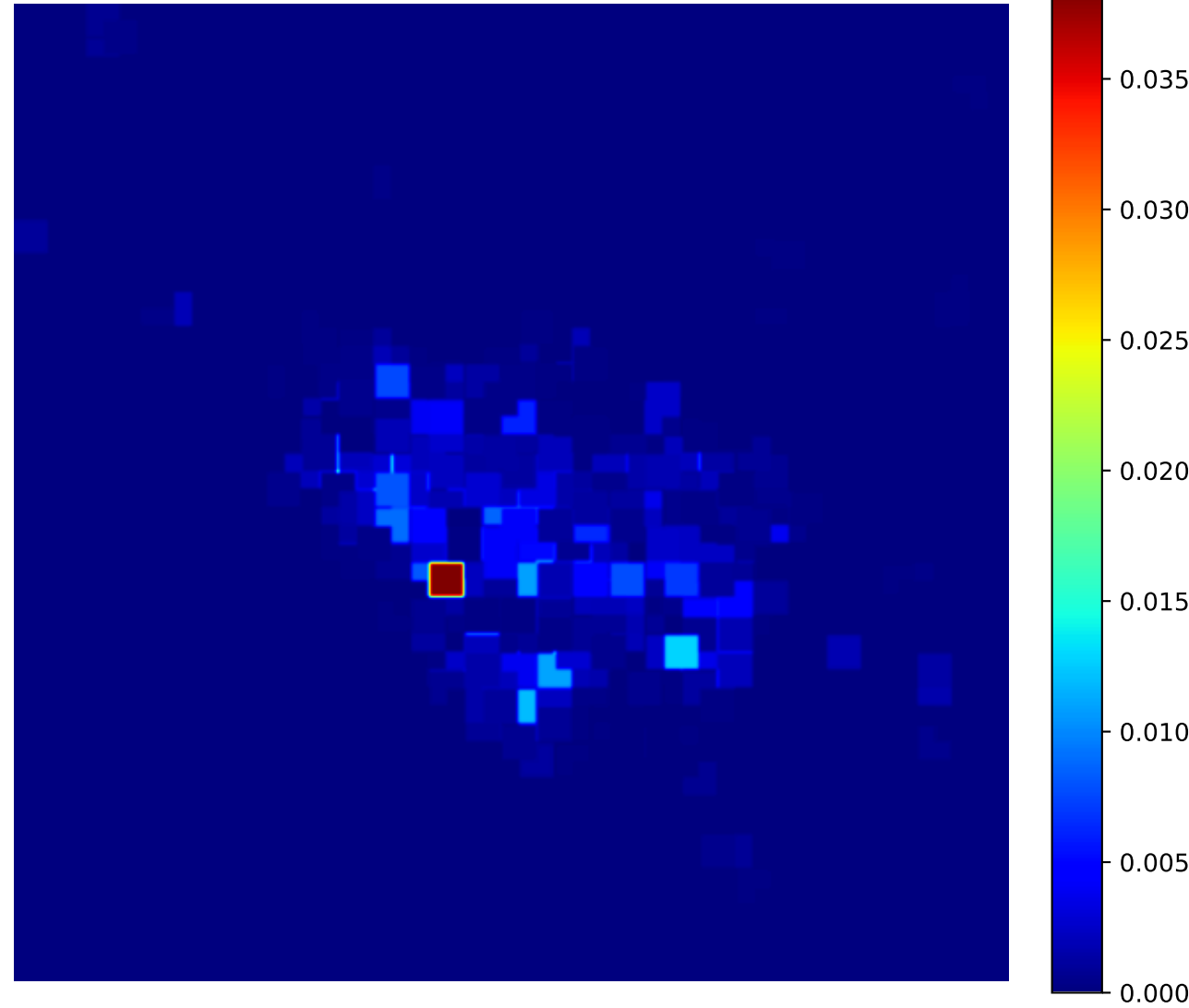
Attention Heatmap
